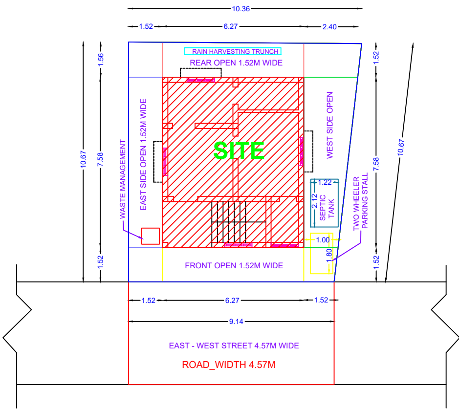
SITE PLAN
