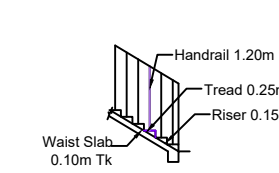
DETAILS OF STAIR CASE (SCALE 1:100)
