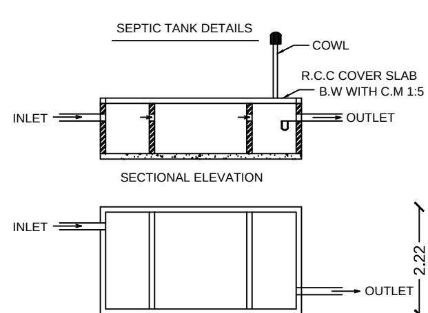
PLAN OF SEPTIC TANK
