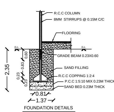
FOUNDATION DETAILS
