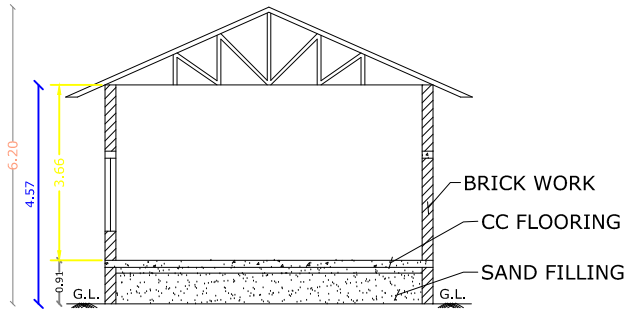
SELECTION ON "AA"
