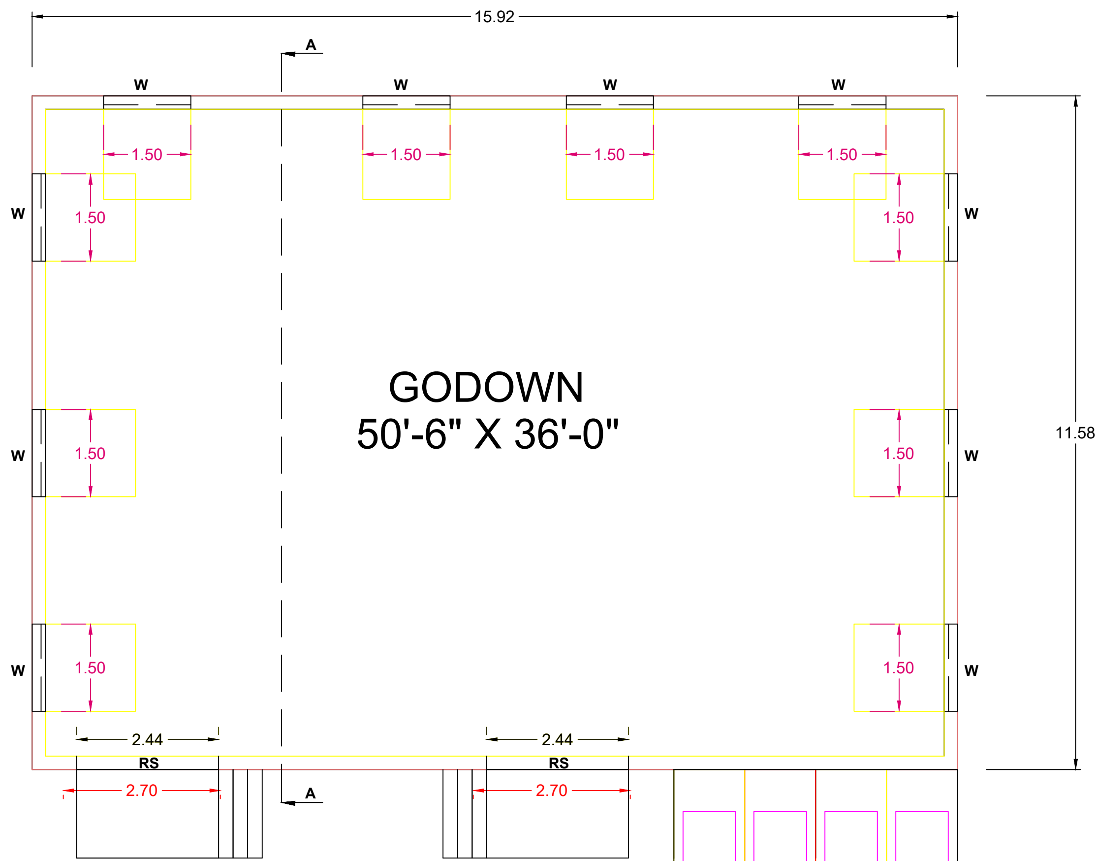
GROUND FLOOR
