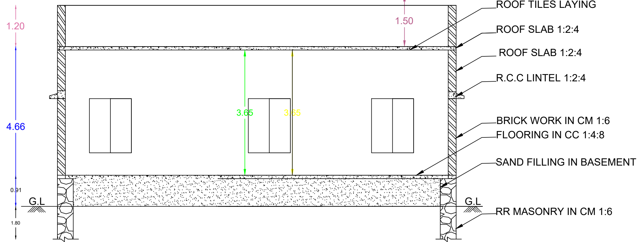
SECTION - AA
