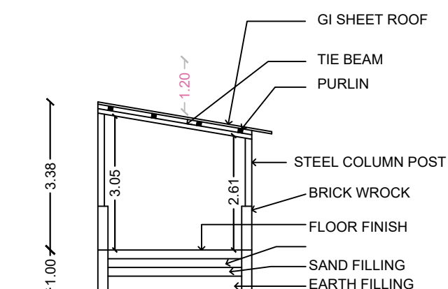
SECTION ON "XY"
