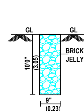
PERCULATION PIT
