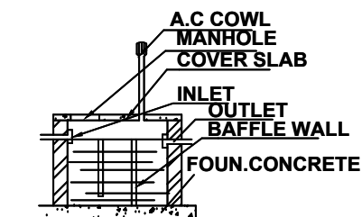
DETAILS OF SEPTIC TANK
