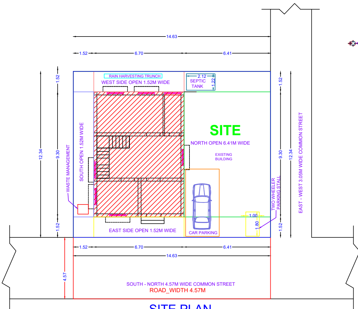
SITE PLAN
