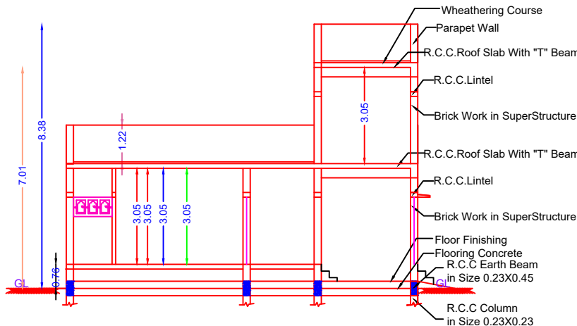
SECTION ON "PQ" (SCALE 1:100)
