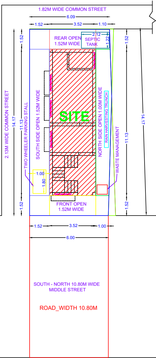
SITE PLAN
