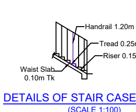
DETAILS OF STAIR CASE (SCALE 1:100)
