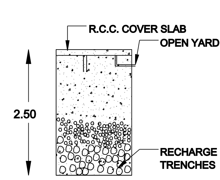
SECTION C-C'
