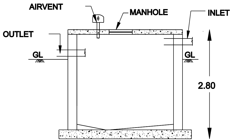
SECTION B-B'
