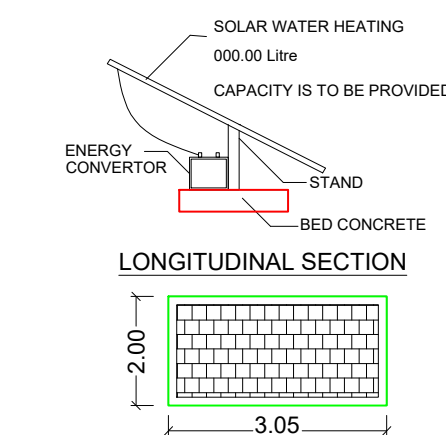
SOLAR SYSTEM
