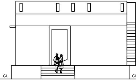
NORTH FACE ELEVATION
