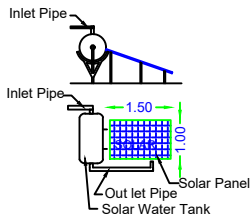
DETAILS OF SOLAR WATER HEATER
