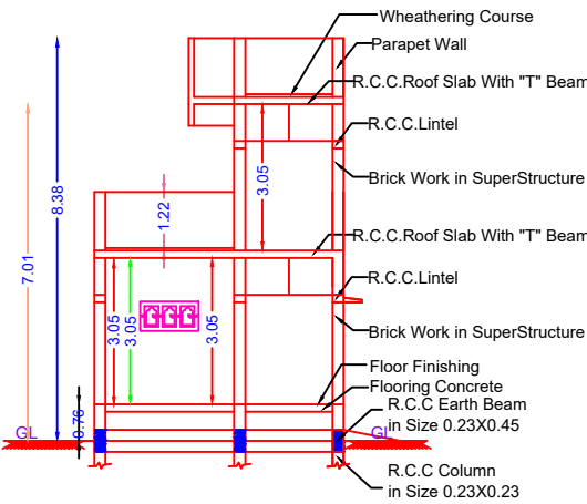
SECTION ON "PQ"
