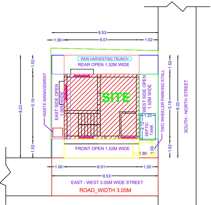
SITE PLAN
