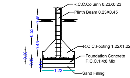
DETAILS OF COLUMN FOOTING
