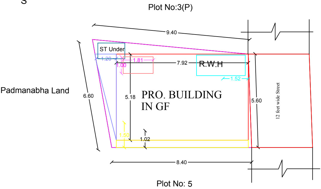
SITE PLAN
