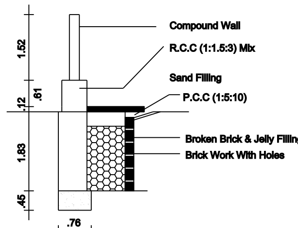
RAIN WATER HARVEST DETAILS
