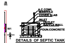
DETAILS OF SEPTIC TANK
