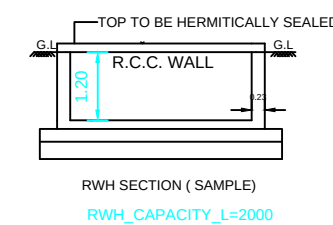
RWH SECTION ( SAMPLE)
