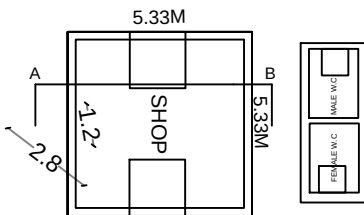
PROPOSED GROUND FLOOR PLAN
