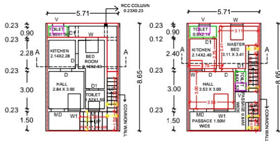
GROUND EXG. AND PRO
