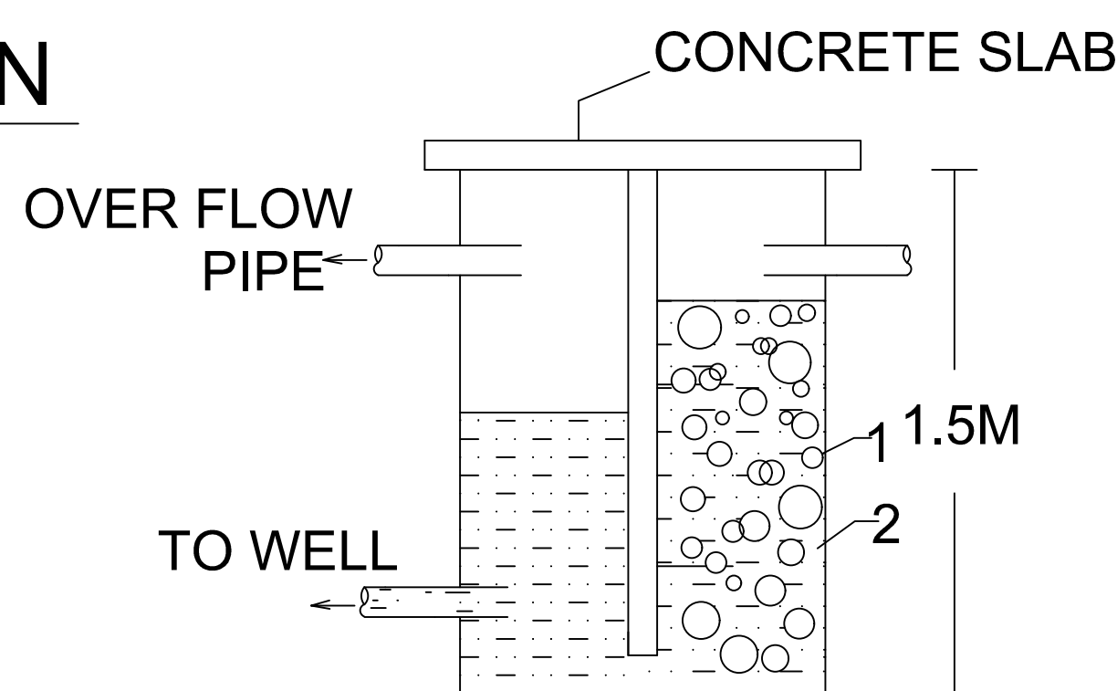
SECTIONS OF R.H.S.
