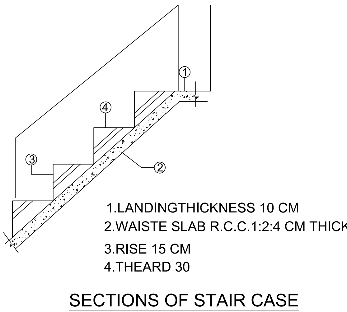
SECTIONS OF STAIR CASE
