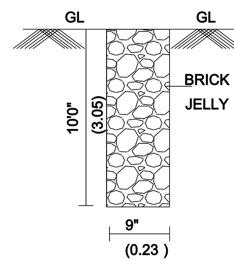
PERCULATION PIT
