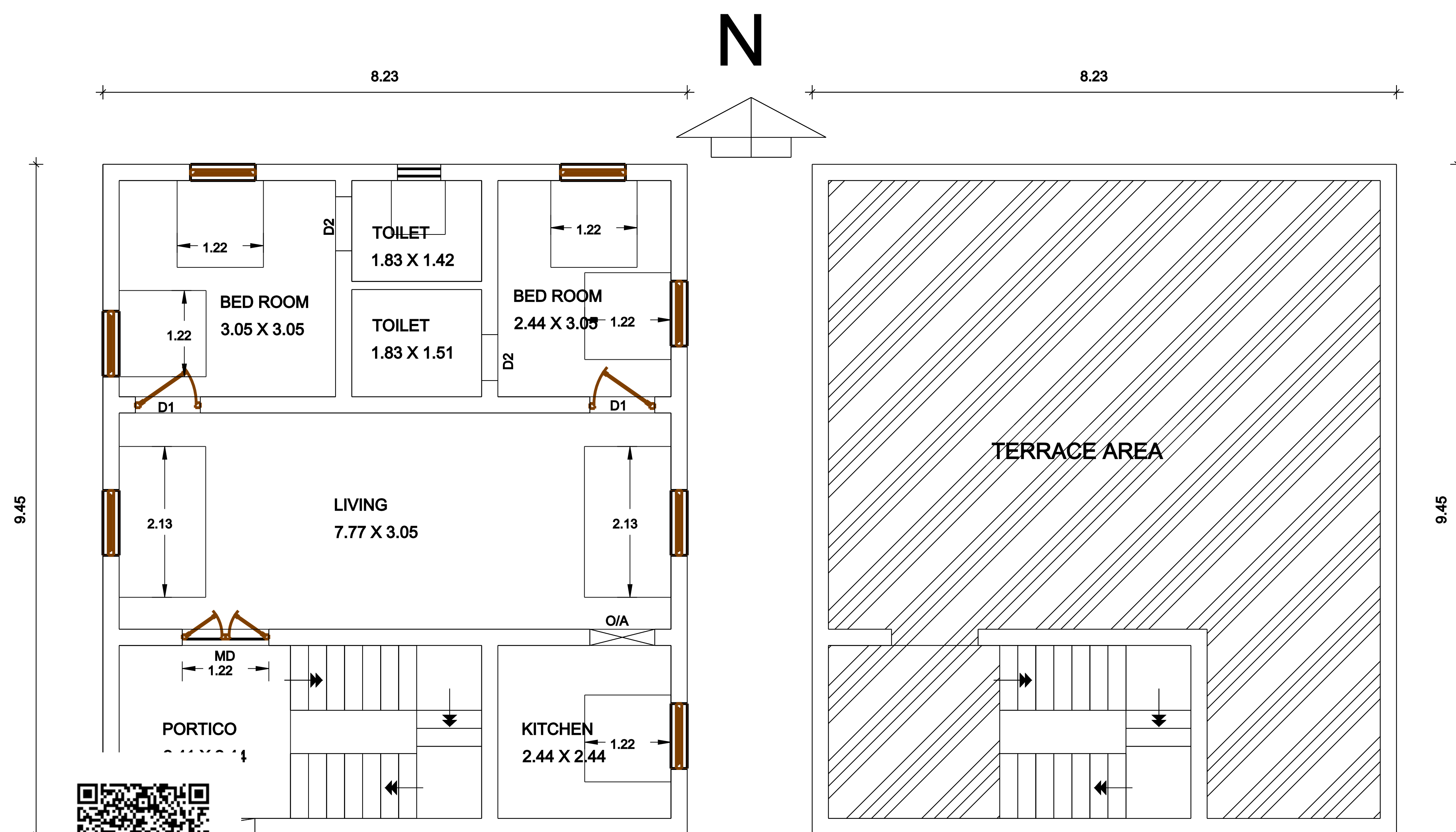
ROUND FLOOR PLAN.
