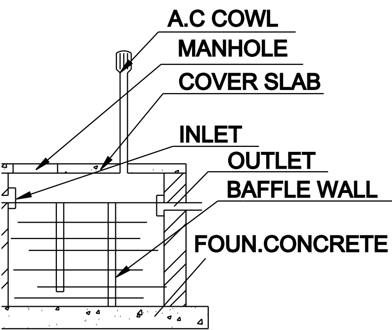
DETAILS OF SEPTIC TANK
