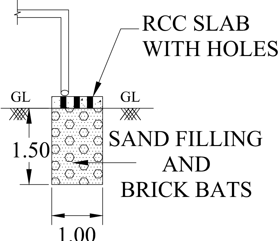
SECTION OF BS
