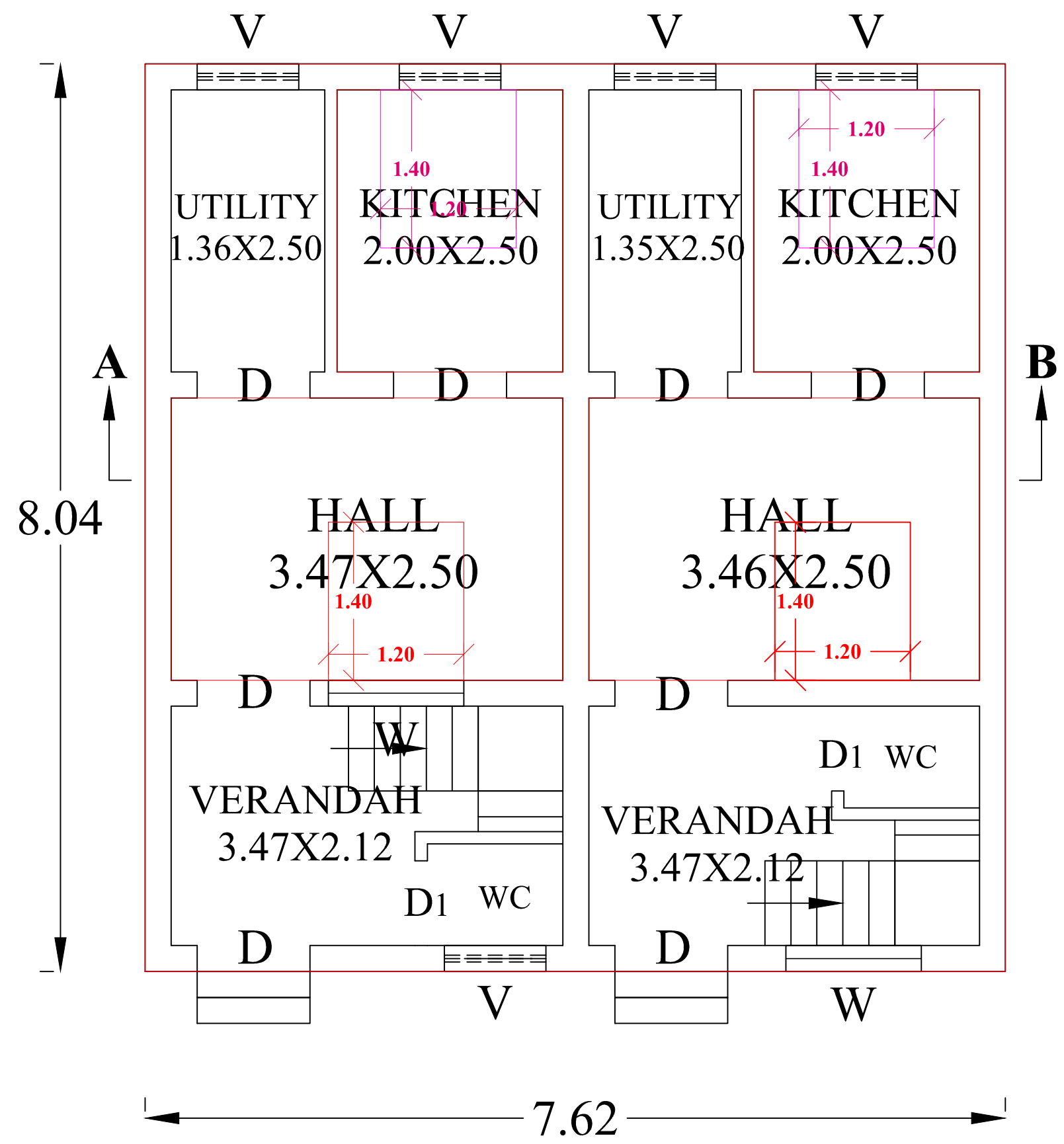
PLAN
