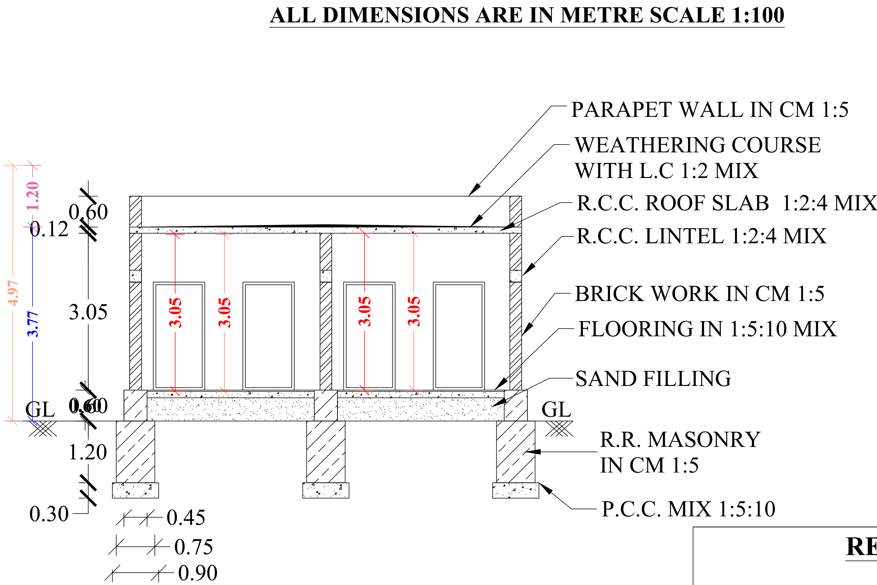
SECTION OF "AB"
