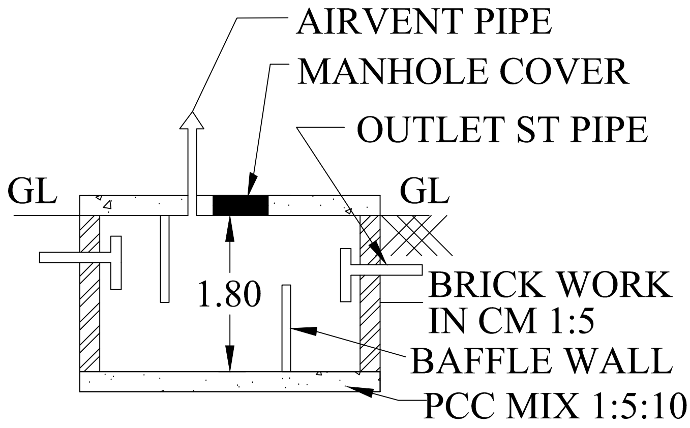
SECTION ON SEPTICTANK
