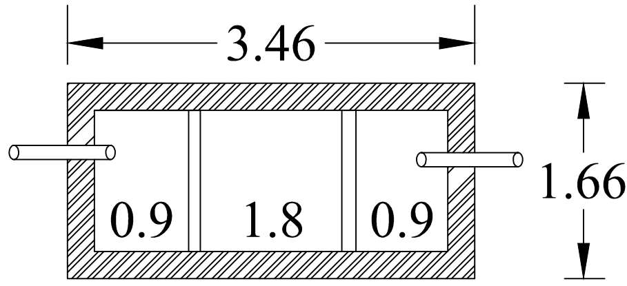
PLAN ON SEPTICTANK
