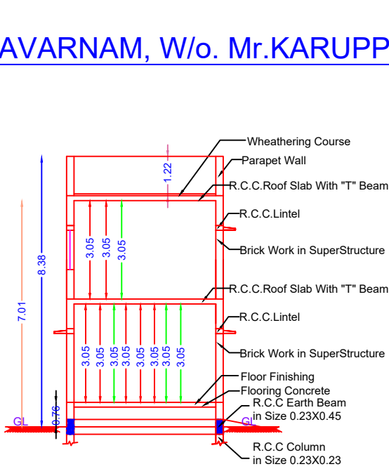
SECTION ON "PQ" (SCALE 1:100)
