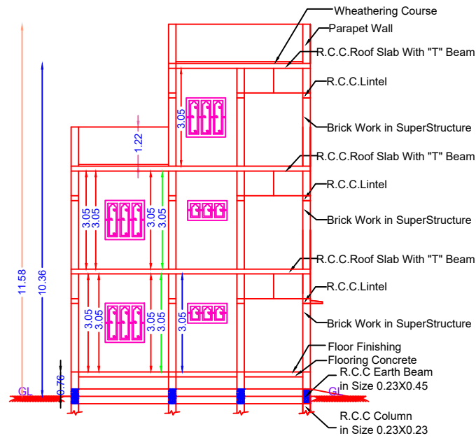
SECTION ON "PQ" (SCALE 1:100)
