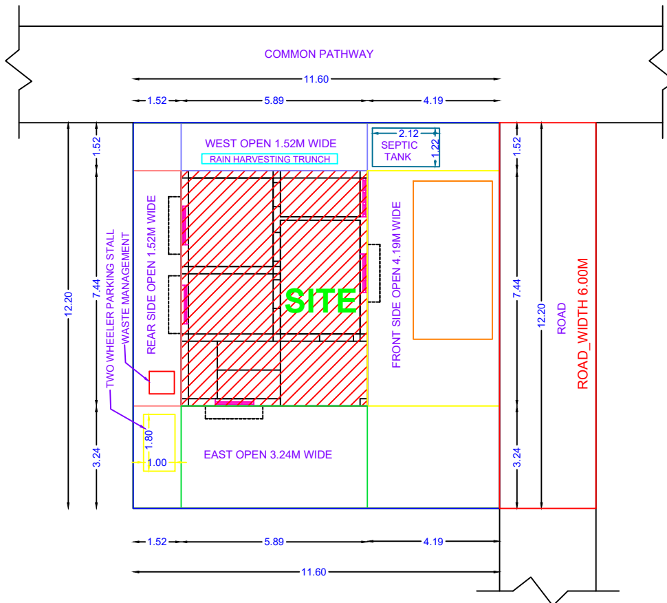
SITE PLAN
