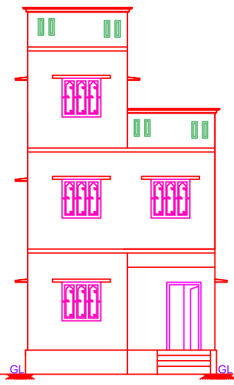
FRONT ELEVATION
