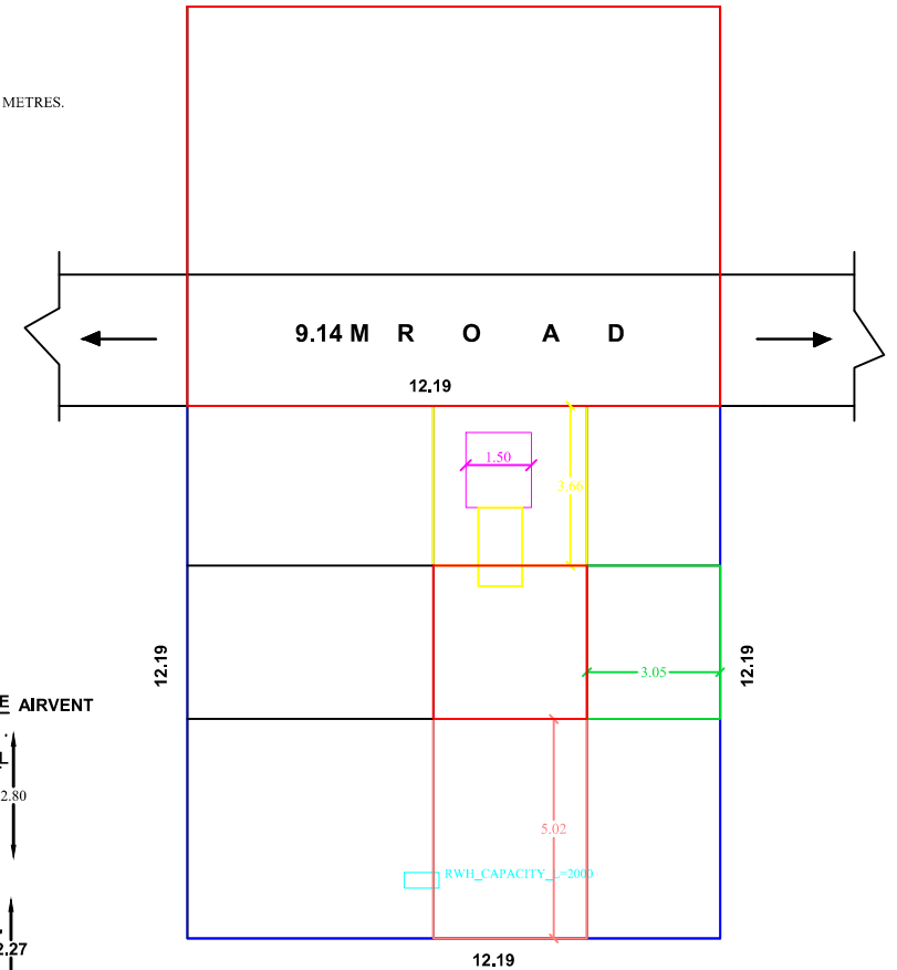
SITE PLAN
