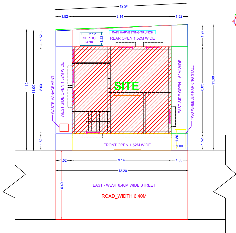
SITE PLAN
