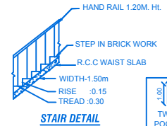
STAIR DETAIL
