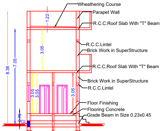
SECTION ON "PQ" SCALE 1:100
