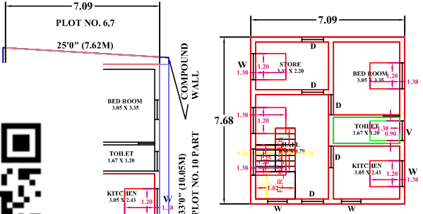
PLAN AT PRO. FIRST FLOOR
