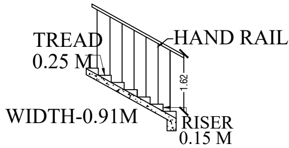
STAIRCASE DETAILS
