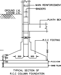
TYPICAL SECTION OF R.C.C. COLUMN FOUNDATION SCALE : 1" = 2'-0"
