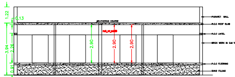
SECTION ON AA
