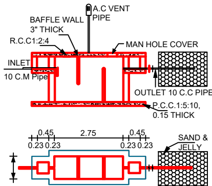
SEPTIC TANK AND TRECH
