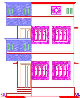
FRONT ELEVATION
