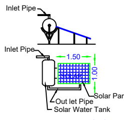
DETAILS OF SOLAR WATER HEATER
