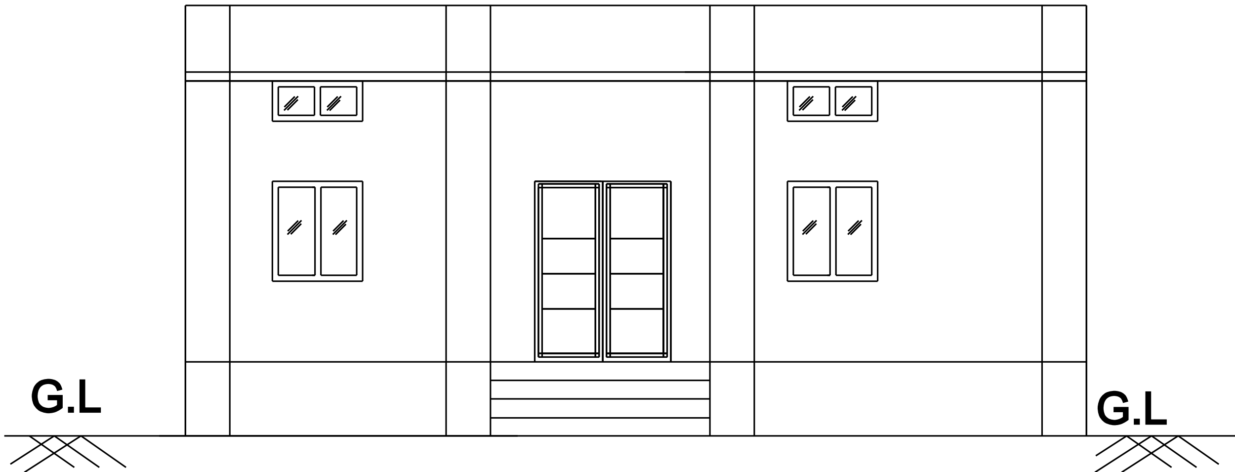
FRONT ELEVATION
