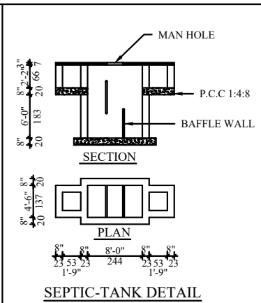
SEPTIC-TANK DETAIL
