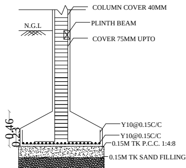
SECTION AT XX
