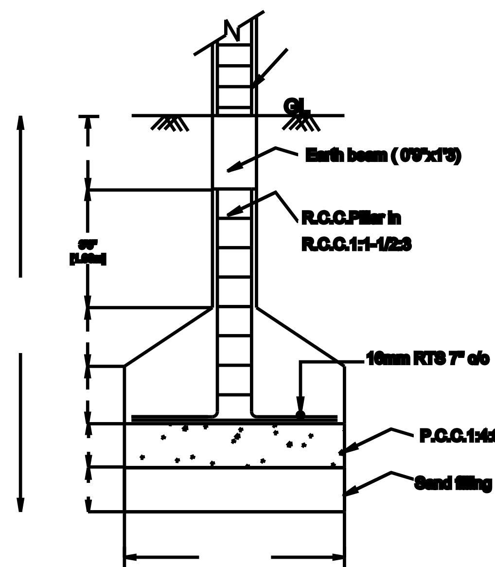
FOUNDATION DETAILS
