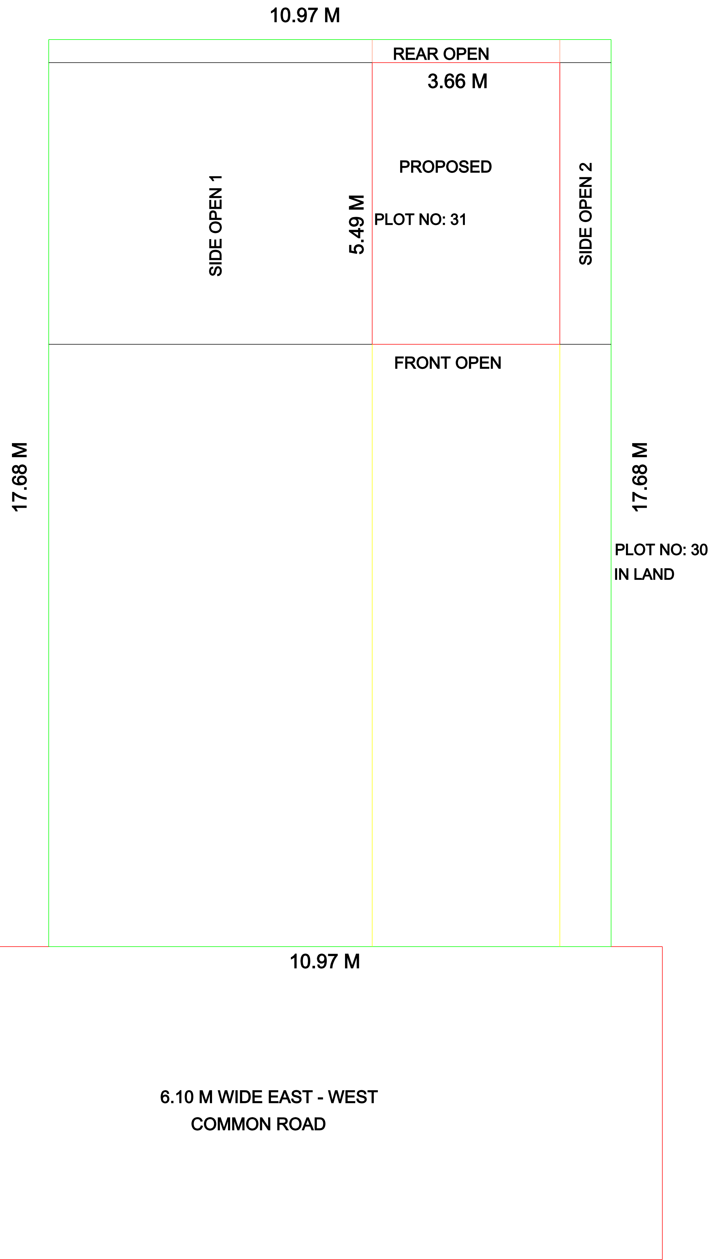
SITE PLAN
