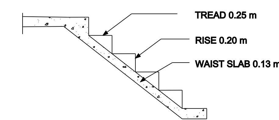
STAIR DETAILS
