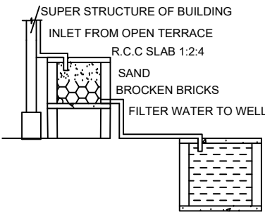
RAINWATER HARVESTING
