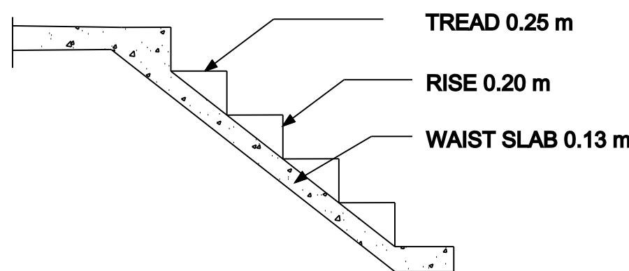
STAIR DETAILS
