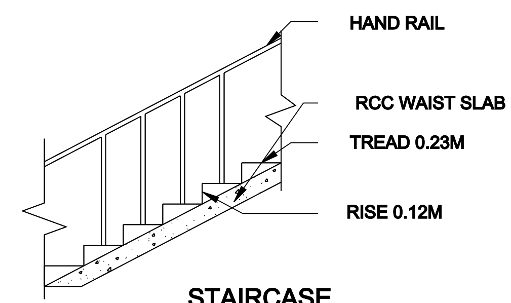
STAIRCASE
