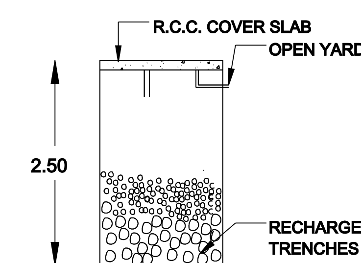
SECTION C-C'
