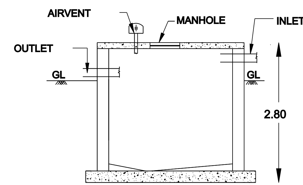
SECTION B-B'
