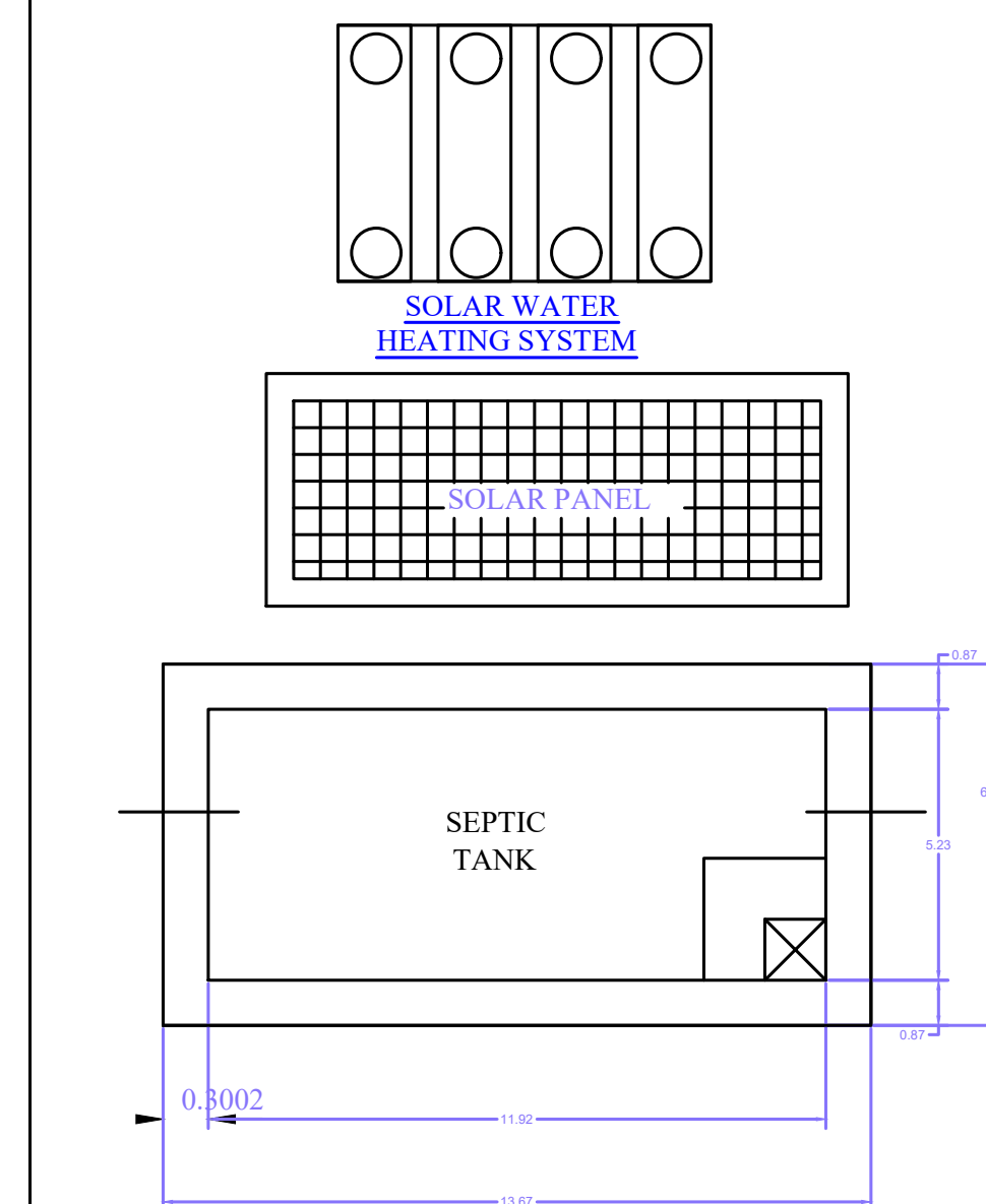
PLAN OF SEPTIC TANK SCALE 1"-2'0"
