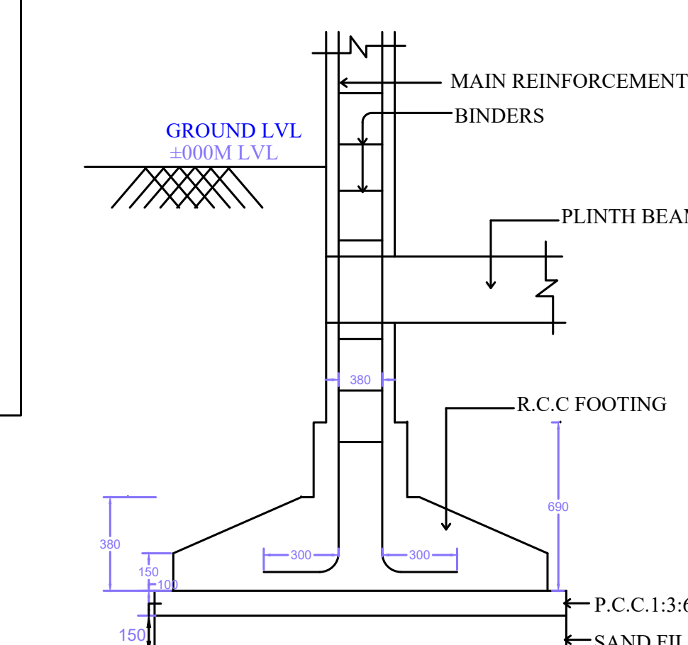
TYPICAL SECTION OF R.C.C COLUMN FOUNDATION SCALE : 1" = 2'-0"
