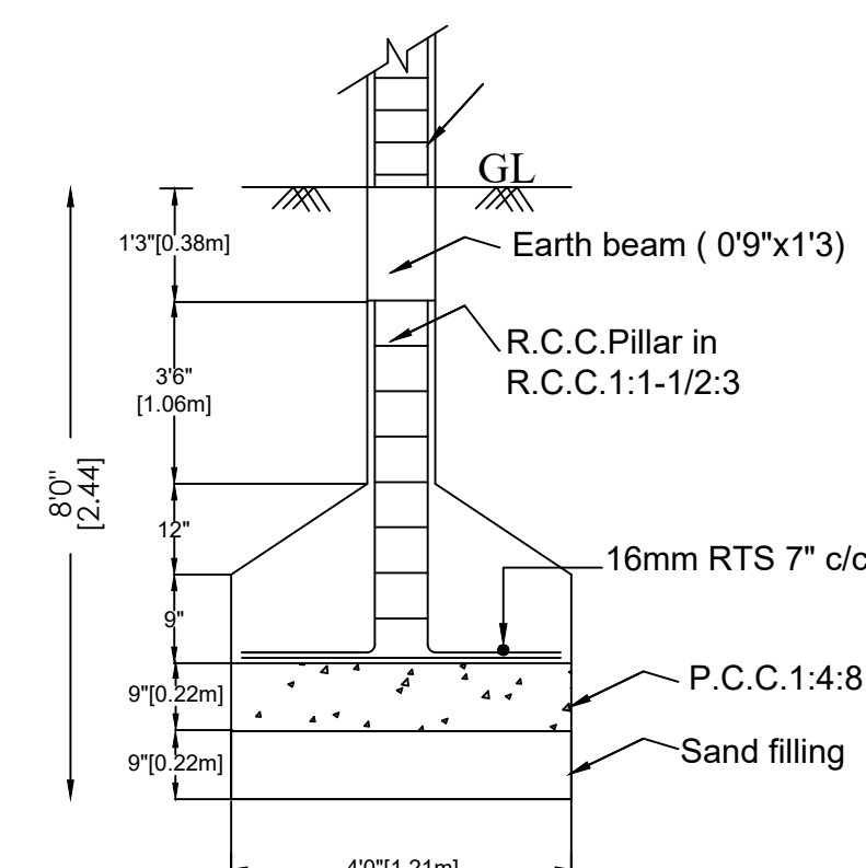
FOUNDATION DETAILS
