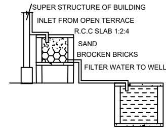
RAINWATER HARVESTING
