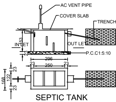
SEPTIC TANK
