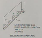
SECTIONS OF STAIR CASE
