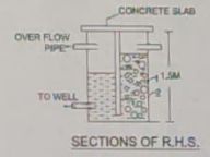
SECTIONS OF R.H.S.
