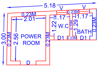
PROPOSED GROUND FLOOR TOILET AREA
