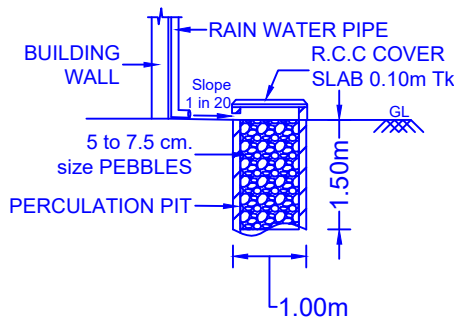
RAIN WATER HARVESTING TRENCH PIT DETAILS
