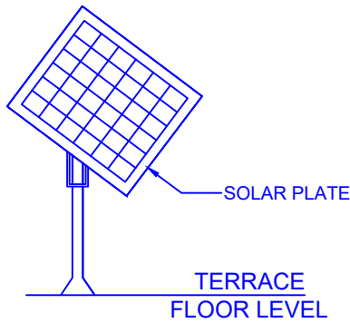
SOLAR SYSTEM
