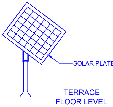
SOLAR SYSTEM
