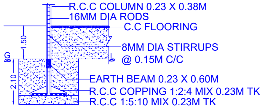
R.C.C COLUMN 0.23 X 0.38M DETAILS
