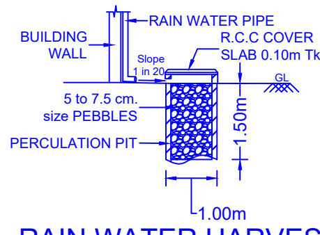
RAIN WATER HARVESTING TRENCH PIT DETAILS
