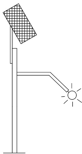
SOLAR SYSTEM
