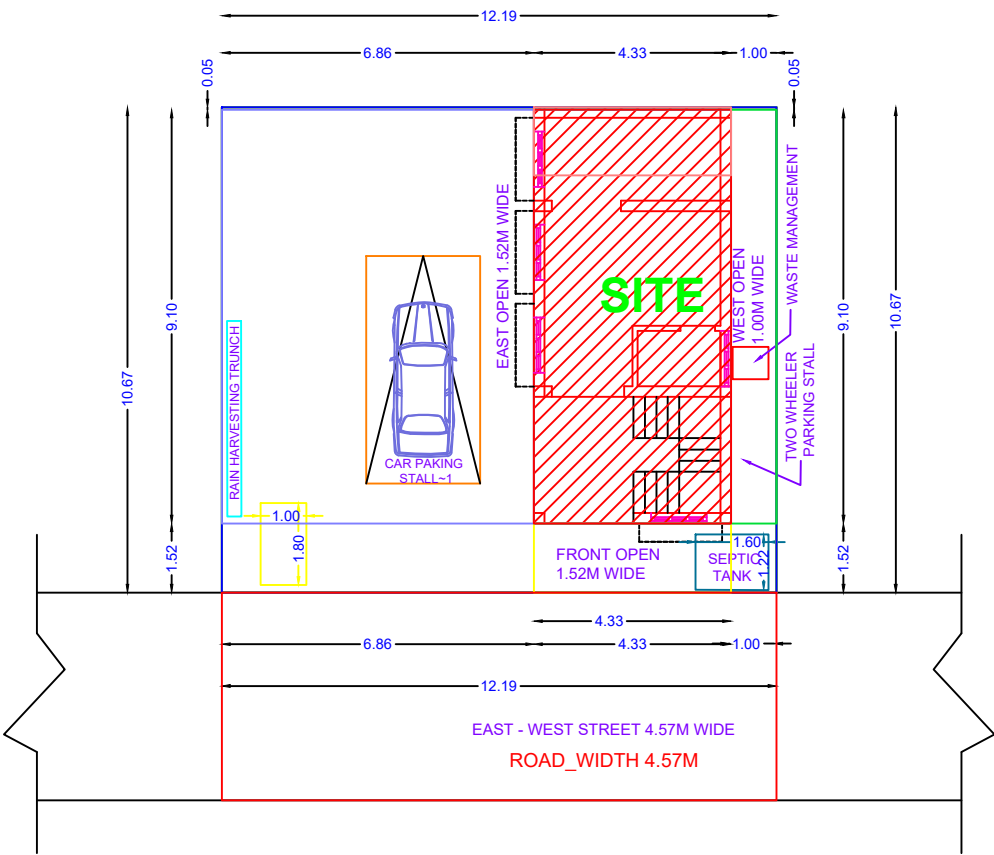
SITE PLAN
